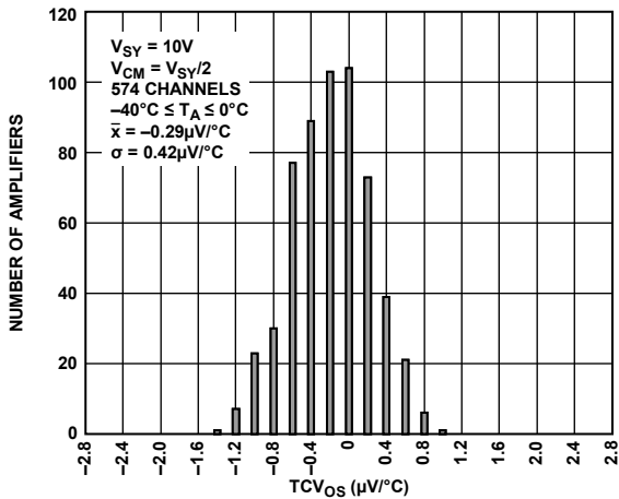
Figure 11. Input Offset Voltage Drift Distribution, -40^{\circ}C \leq T_A \leq 0^{\circ}C , V_{SY} = 10V
