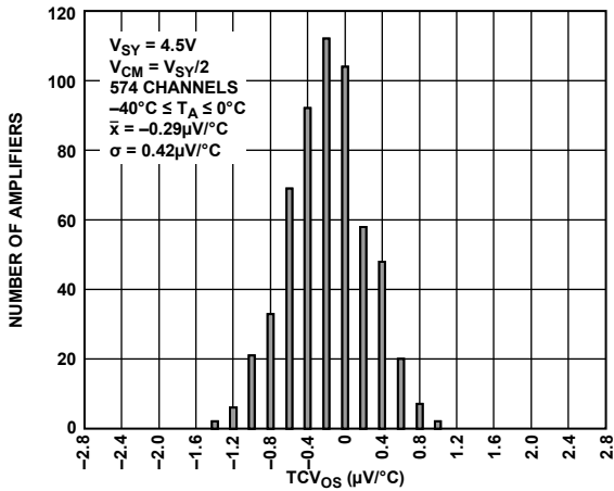
Figure 10. Input Offset Voltage Drift Distribution, -40^{\circ}C \leq T_A \leq 0^{\circ}C , V_{SY} = 4.5V
