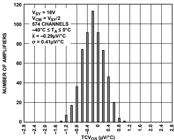
Figure 12. Input Offset Voltage Drift Distribution, -40^{\circ}C \leq T_A \leq 0^{\circ}C , V_{SY} = 16V
