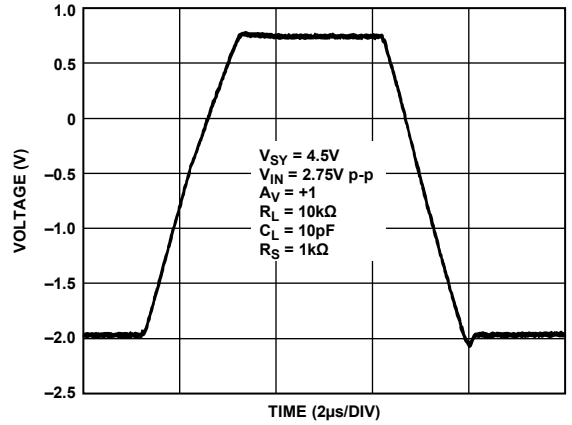
Figure 64. Large Signal Transient Response, V_{SV} = 4.5 V
