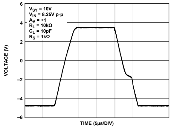
Figure 65. Large Signal Transient Response, V_{SV} = 10 V
