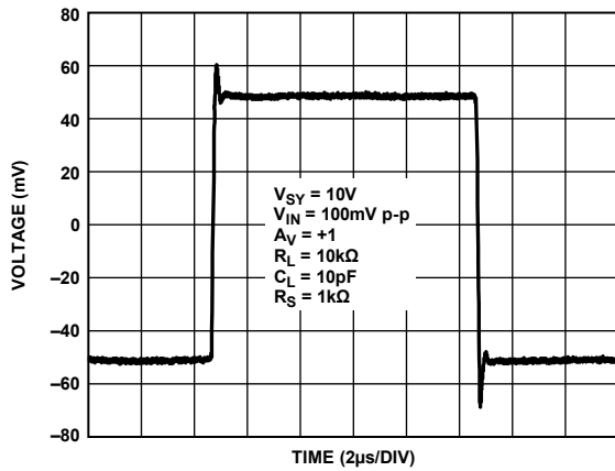
Figure 62. Small Signal Transient Response, V_{SV} = 10 V
