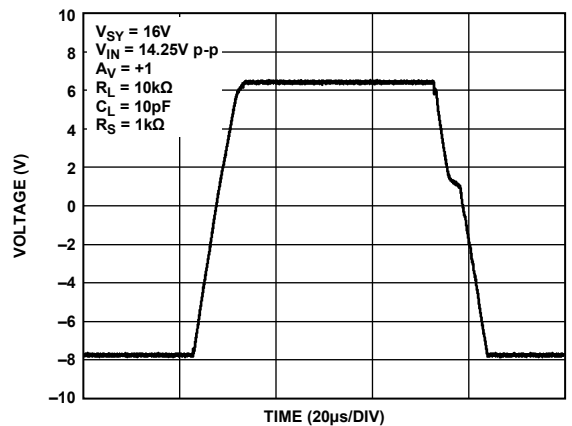
Figure 66. Large Signal Transient Response, V_{SV} = 16 V
