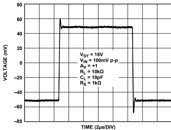
Figure 63. Small Signal Transient Response, V_{SV} = 16 V
