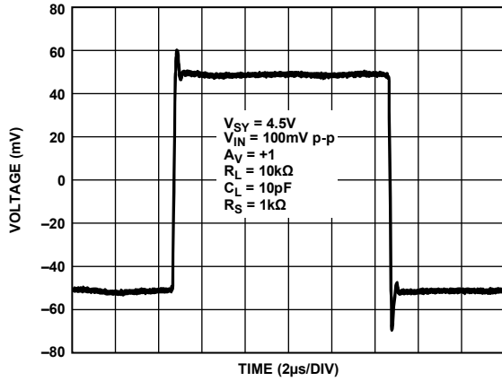
Figure 61. Small Signal Transient Response, V_{SV} = 4.5 V
