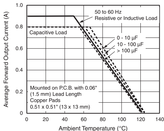
Fig. 2 - Derating Curves Output Rectified Current for B250C800DM...B360C800DM
