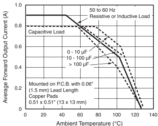
Fig. 1 - Derating Curves Output Rectified Current for B40C800DM...B125C800DM
