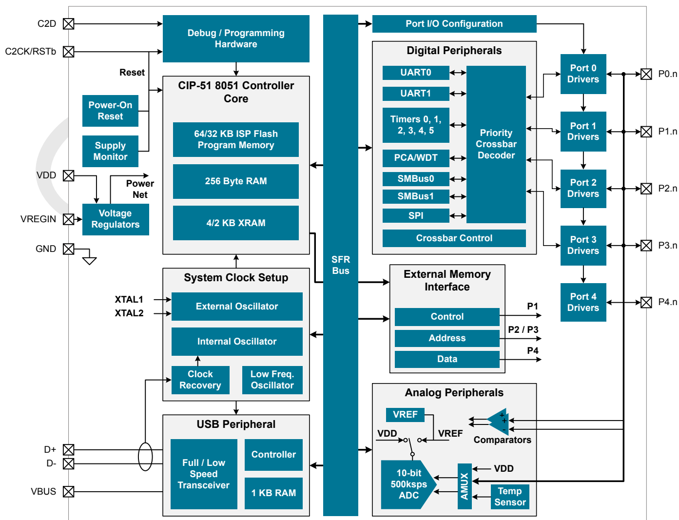
Figure 2.1. Detailed EFM8UB2 Block Diagram
