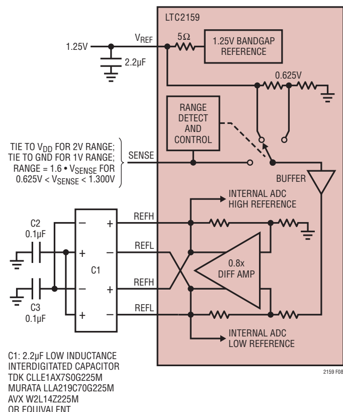
Figure 8a. Reference Circuit
