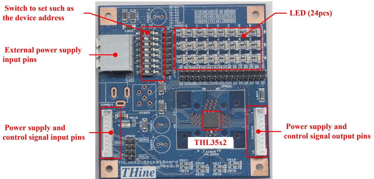
Figure 1 Board Overview
