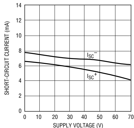
Driver Short-Circuit Current vs Supply Voltage
