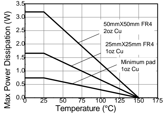
Derating Curve
