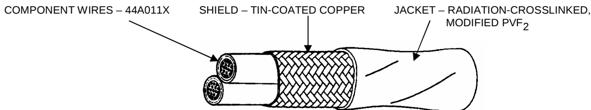
CABLE CONSTRUCTION DETAILS
