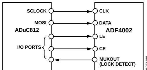
Figure 22. ADuC812 to ADF4002 Interface
