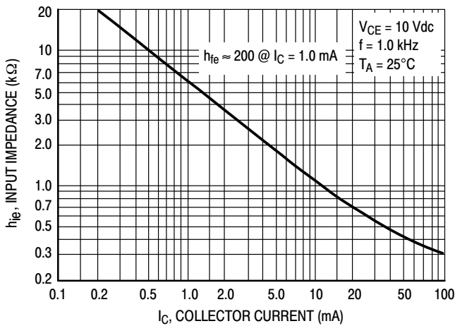
Figure 18. Input Impedance
