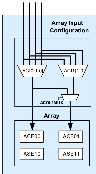
Figure 2. CY8C21x23 Analog System Block Diagram
