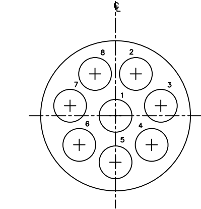
12-08 8 #16 CAVITIES
