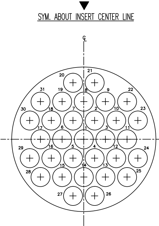
20-31 31 #16 CAVITIES
