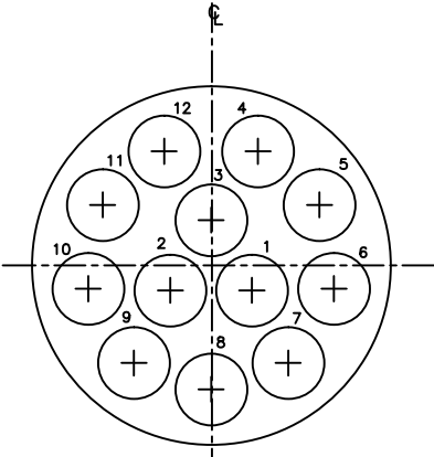
14-12 12 #16 CAVITIES
