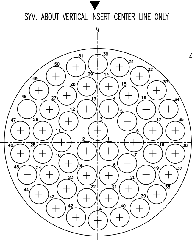
24-51 51 #16 CAVITIES
