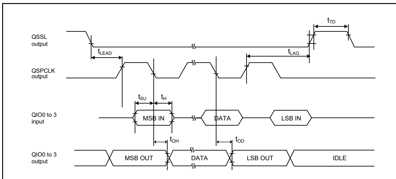
Figure 2.69 Transfer/receive timing
