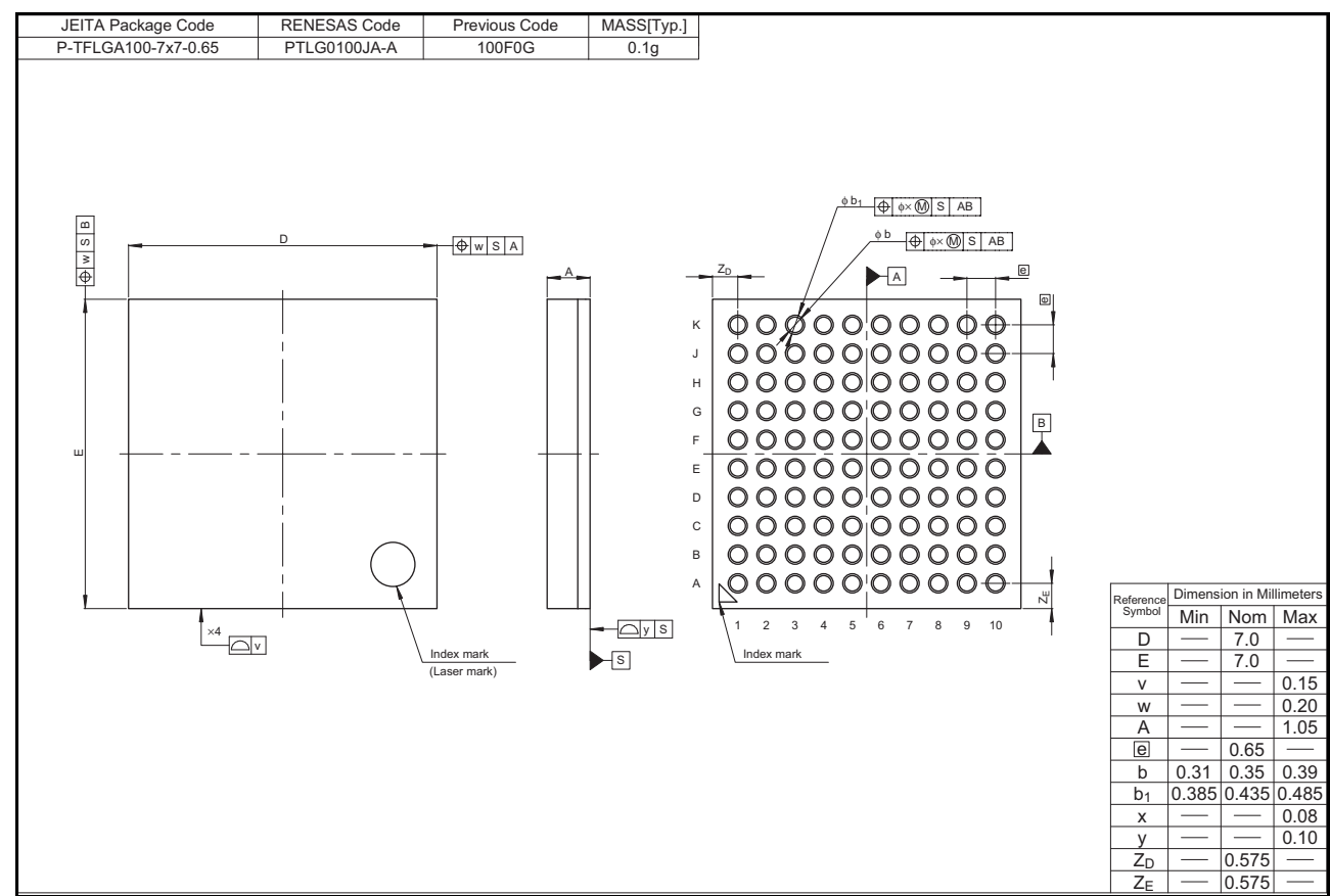
Figure 1.4 LGA 100-pin
