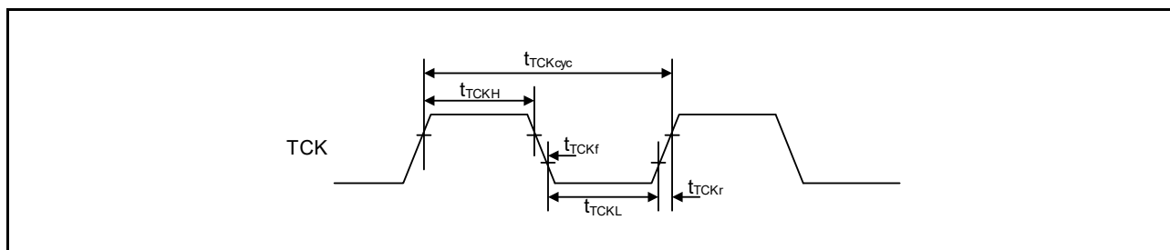
Figure 2.94 Boundary scan TCK timing
