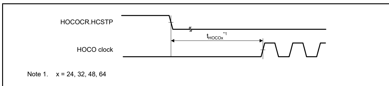
Figure 2.29 HOCO clock oscillator start timing (started by setting HOCOOCR.HCSTP bit)
