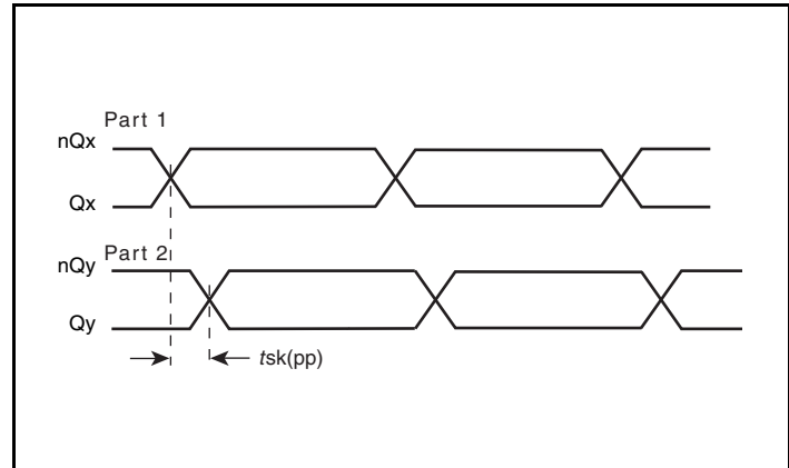
Part-to-Part Skew
