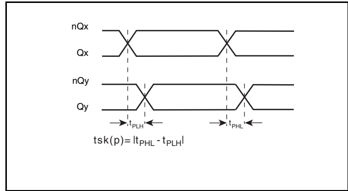
Pulse Skew
