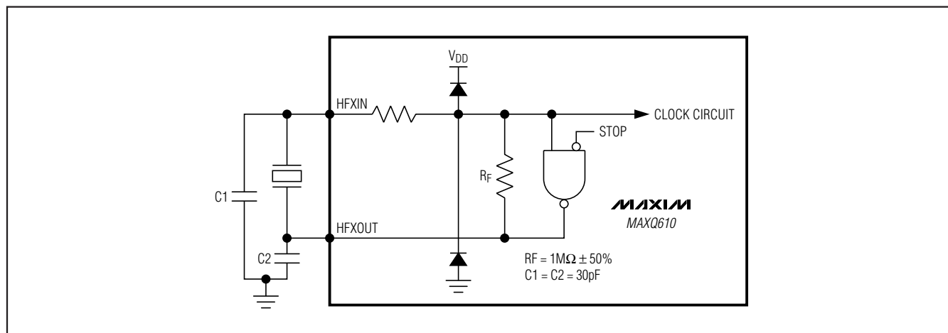
Figure 9. On-Chip Oscillator
