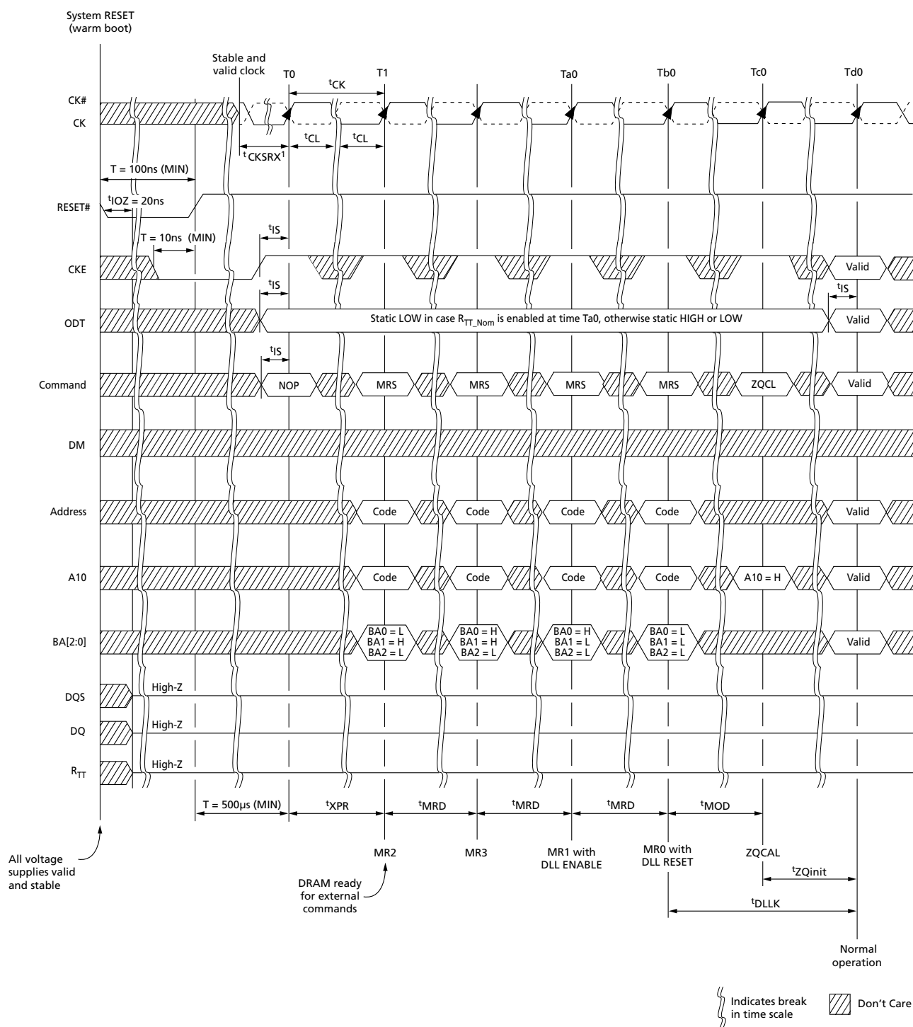
Figure 105: RESET Sequence
