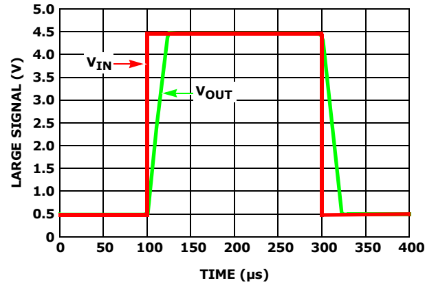
FIGURE 44. SIMULATED LARGE SIGNAL STEP RESPONSE (4V)
