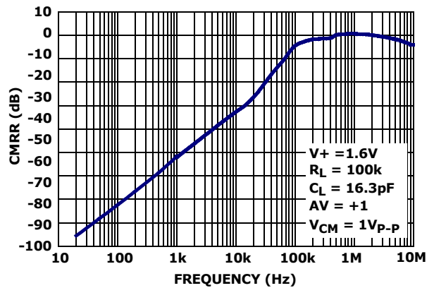
FIGURE 24. CMRR vs FREQUENCY, V_S = 1.6V
