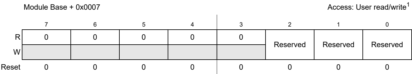
Figure 12-7. Reserved Register
