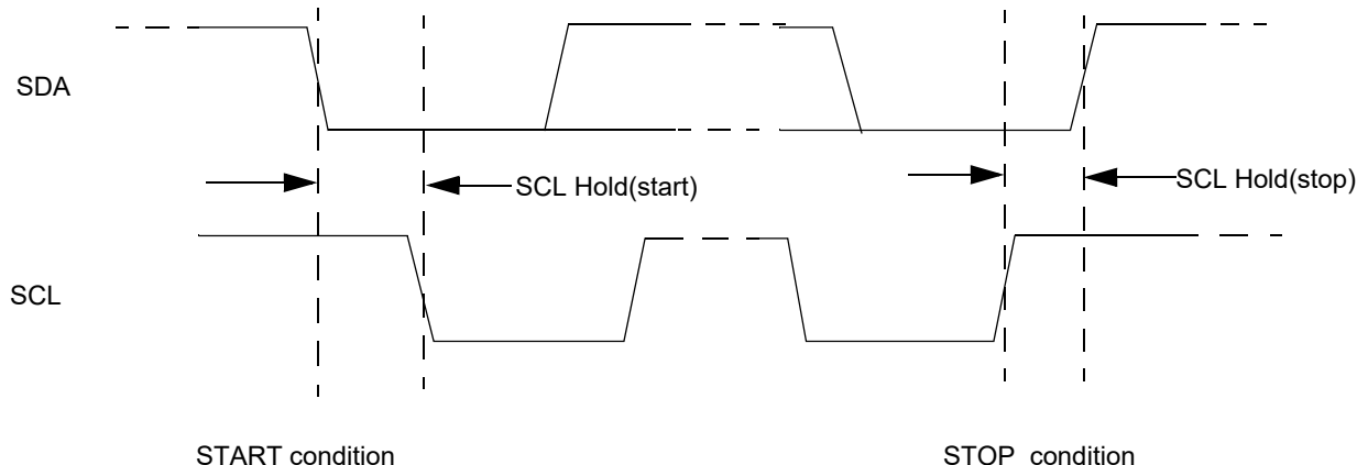
Figure 20-5. SCL Divider and SDA Hold
