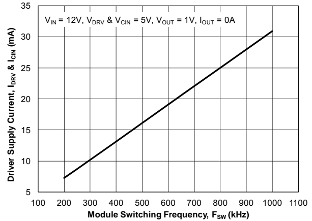
Figure 15. Driver Supply Current vs. Switching Frequency
