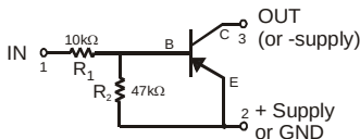
Device Symbol
