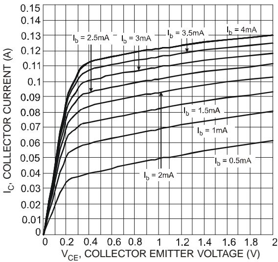
Fig. 18 Typical V_{CE} vs. I_C
