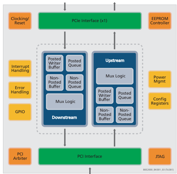
Figure 1 Block Diagram
