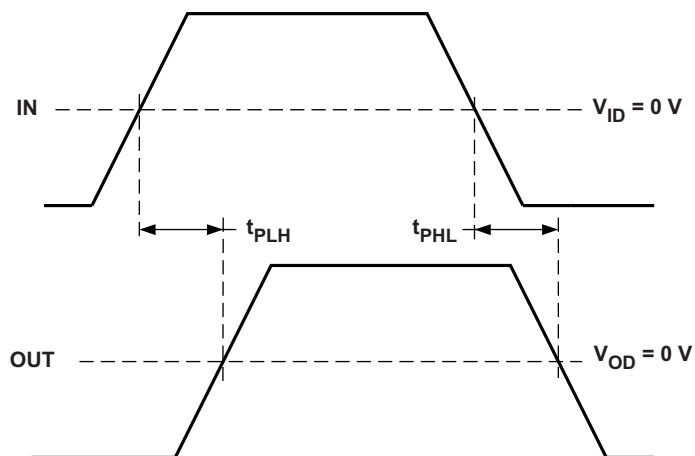
Figure 6. Propagation Delay Input to Output
