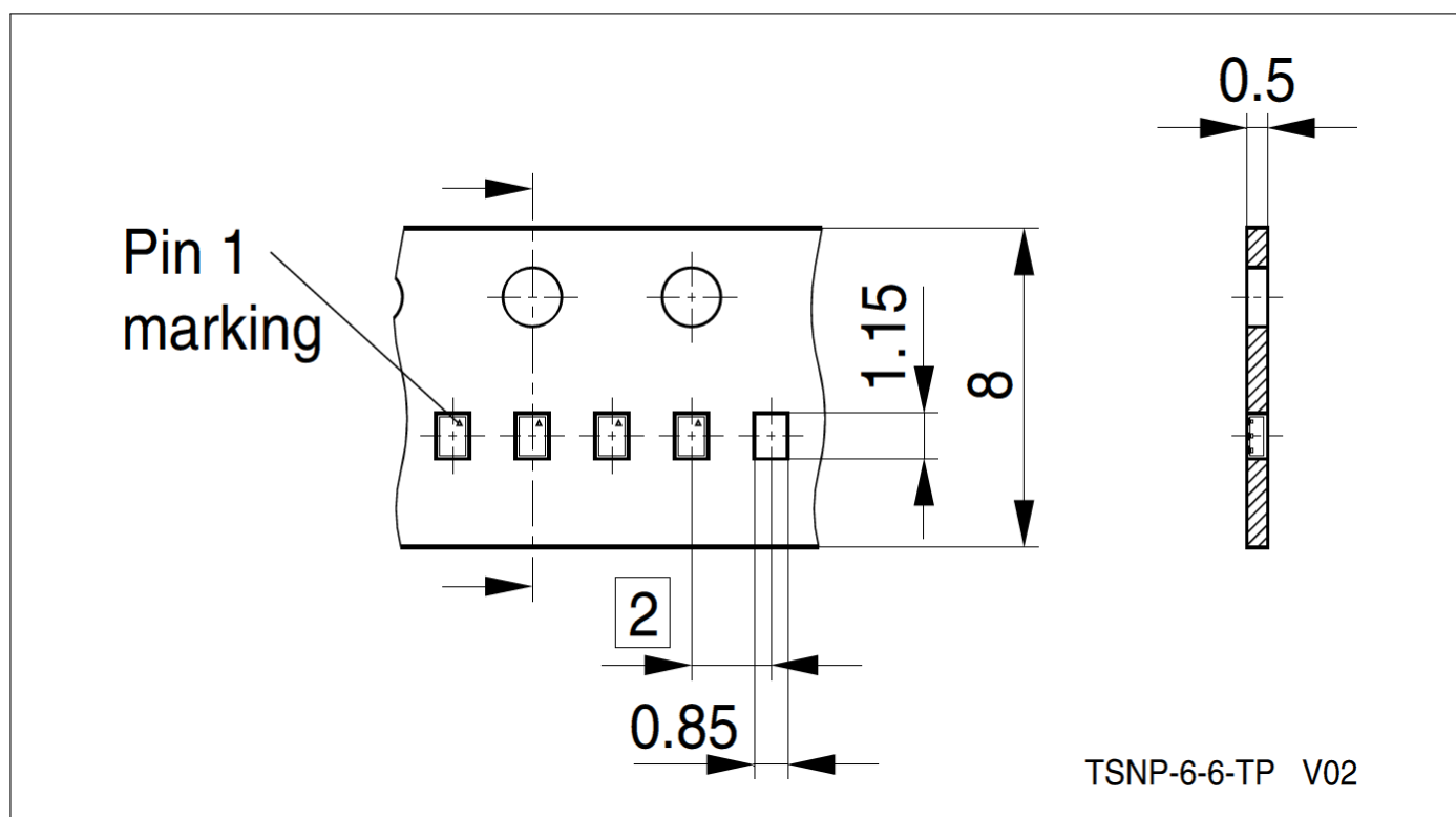
Figure 6: Tape Drawing for TSNP6-6
