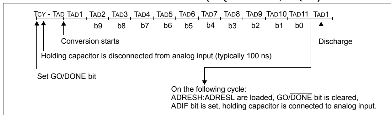
FIGURE 20-4: A/D CONVERSION TAD CYCLES (ACQT<2:0> = 000, Tacq = 0)
