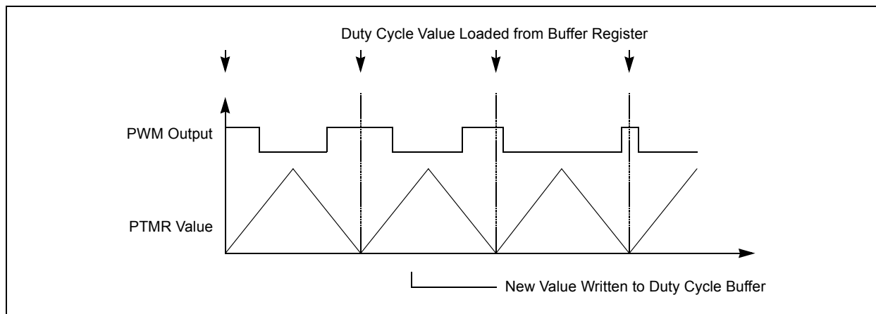
FIGURE 18-13: DUTY CYCLE UPDATE TIMES IN CONTINUOUS UP/DOWN COUNT MODE
