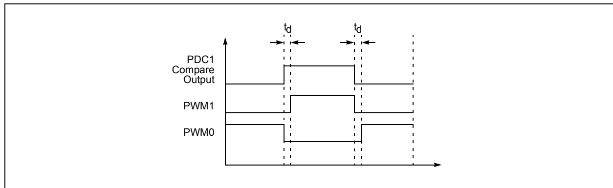
FIGURE 18-18: DEAD-TIME INSERTION FOR COMPLEMENTARY PWM
