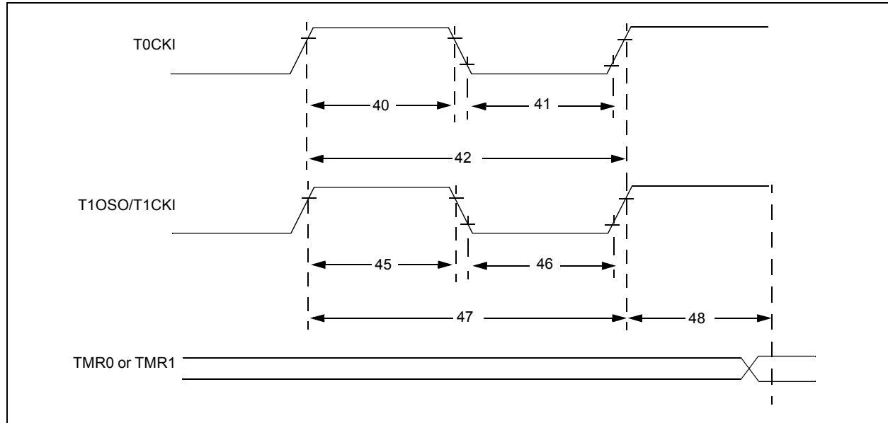
FIGURE 26-9: TIMER0 AND TIMER1 EXTERNAL CLOCK TIMINGS
