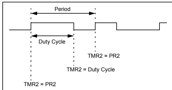
FIGURE 16-4: PWM OUTPUT
