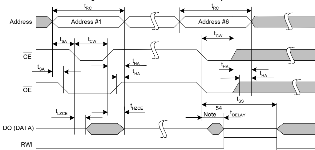
Figure 14. AutoStore Enable/Disable Cycle [51]
