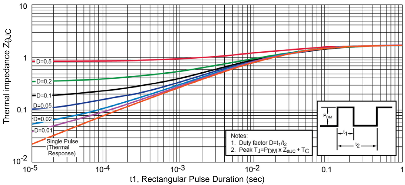
FIGURE 4 Thermal Impedance Curves
