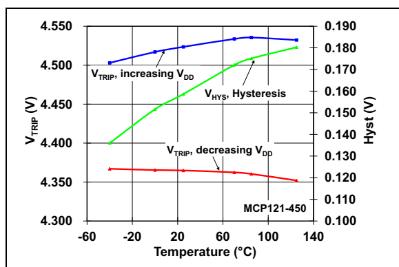
FIGURE 2-15: V_{TRIP} vs. Temperature vs. Hysteresis (MCP121-450).
