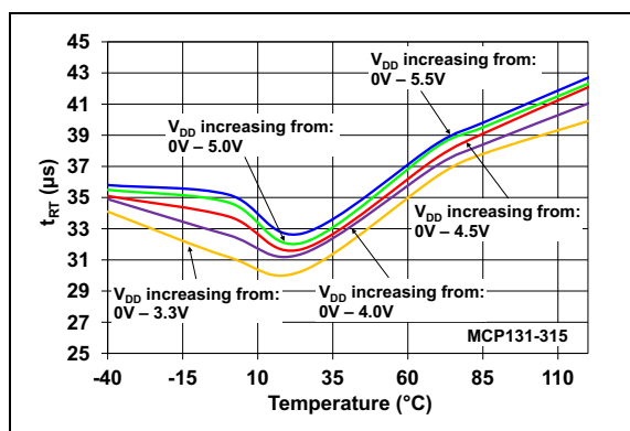
FIGURE 2-30: t_{RT} vs. Temperature (MCP131-315).
