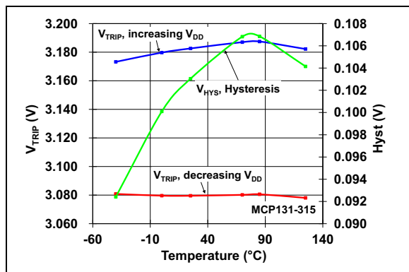
FIGURE 2-14: V_{TRIP} vs. Temperature vs. Hysteresis (MCP131-315).
