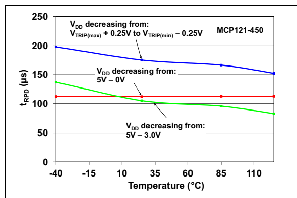
FIGURE 2-25: t_{RPD} vs. Temperature (MCP121-450).
