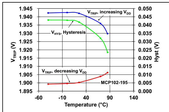
FIGURE 2-13: V_{TRIP} vs. Temperature vs. Hysteresis (MCP102-195).
