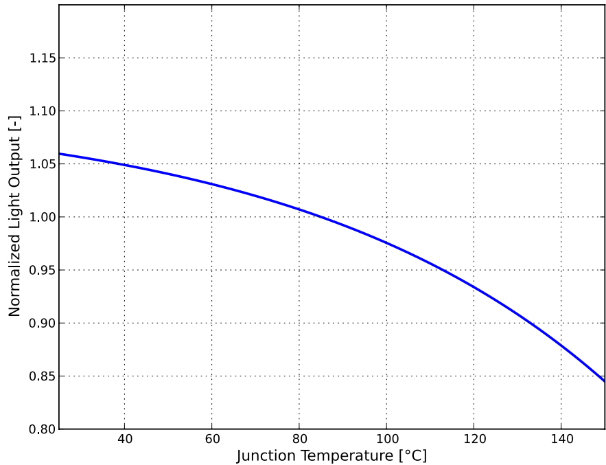
Figure 7. Typical relative light output vs. junction temperature, LIT2-xyyy000000000.
