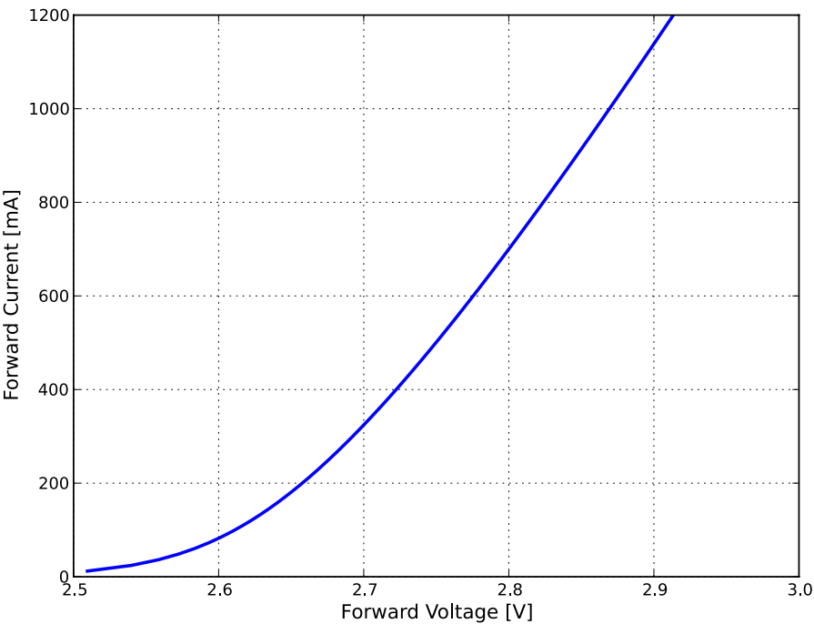
Figure 9. Typical forward current vs. forward voltage, L I T2-xyyy000000000.
