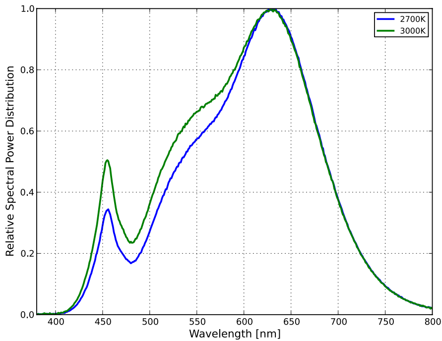
Figure 6. Color Spectrum of LIT2-xx90000000000.
