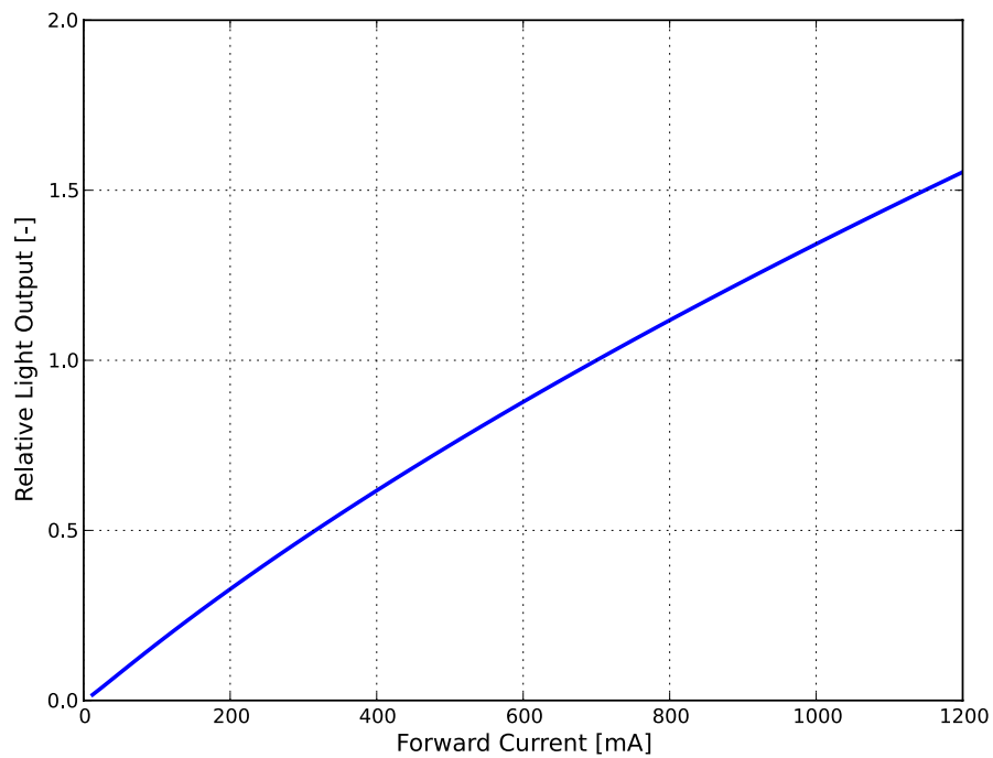
Figure 8. Typical relative luminous flux vs. forward current, LIT2-xyyy000000000.
