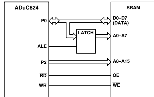
Figure 45. External Data Memory Interface (64 K Address Space)
