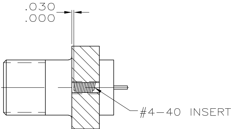
SECTION B-B FOR 861658-1 & -2
