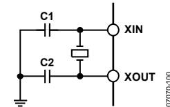
Figure 22. Circuit for Crystal Resonator
