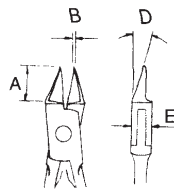
Head Dimensions: A-.55" B-.05" D-13° E-.28"
