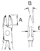
Head Dimensions: A-.55" B-13° E-.28"
