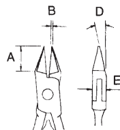
Head Dimensions: A-.55" B-.05" D-14° E-.28"
