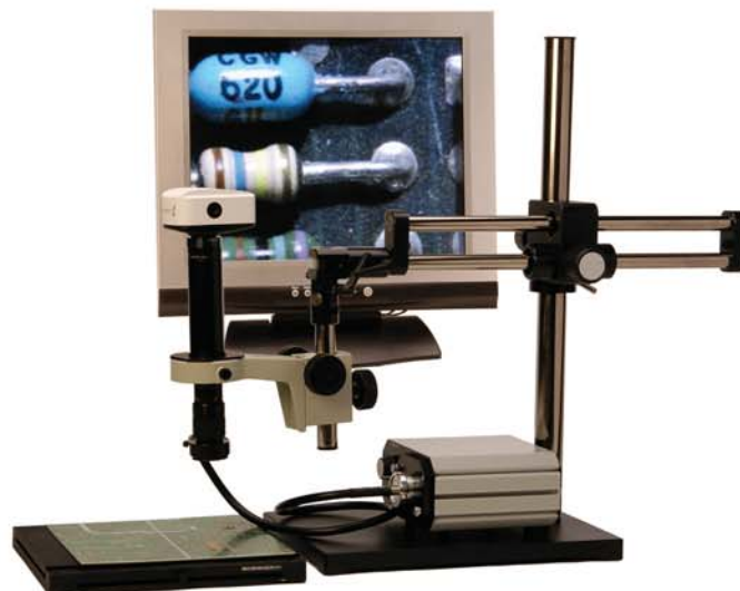
Micro Zoom Video Inspection System on Boom Stand 2700-102-10
