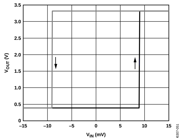
Figure 30. Comparator Hysteresis
