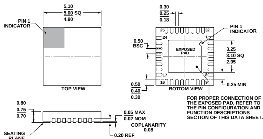
Figure 45. 32-Lead Lead Frame Chip Scale Package [LFCSP_WQ] 5 mm x 5 mm Body, Very Very Thin Quad (CP-32-7)
