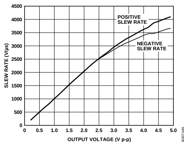
Figure 25. Slew Rate vs. Output Voltage Swing
