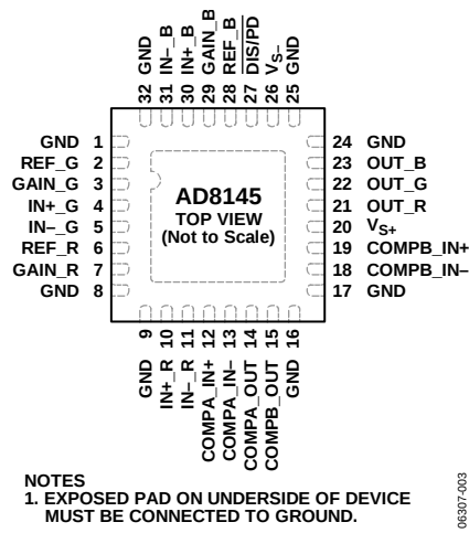
Figure 3. Pin Configuration
