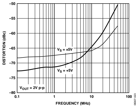
Figure 23. Second Harmonic Distortion vs. Frequency and Power Supplies, V_{OUT} = 2\text{ V p-p} , G = 1
