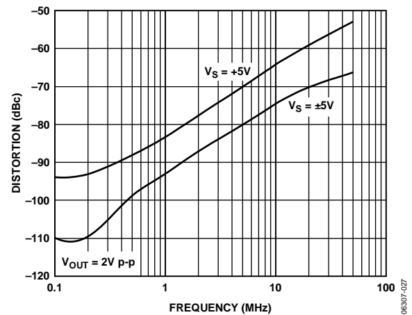
Figure 27. Third Harmonic Distortion vs. Frequency and Power Supplies, V_{OUT} = 2\text{ V p-p} , G = 2
