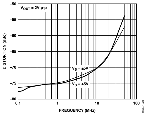
Figure 24. Second Harmonic Distortion vs. Frequency and Power Supplies, V_{OUT} = 2\text{ V p-p} , G = 2
