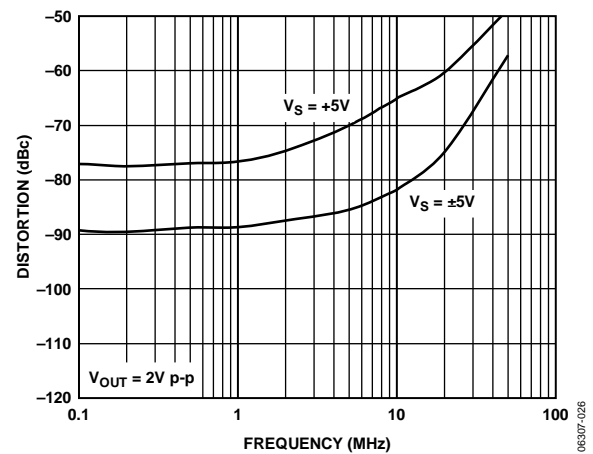
Figure 26. Third Harmonic Distortion vs. Frequency and Power Supplies, V_{OUT} = 2\text{ V p-p} , G = 1
