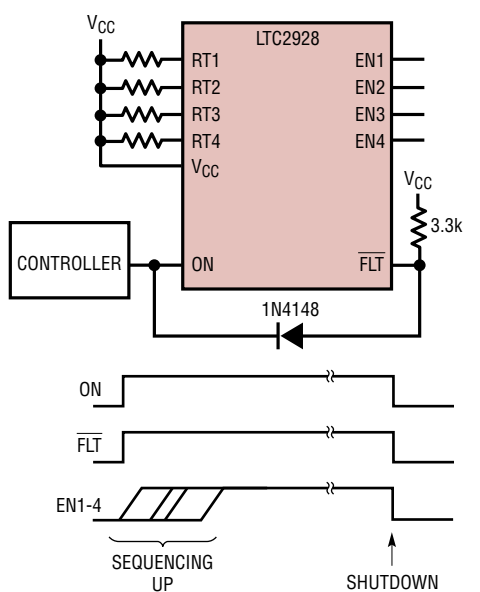
Figure 14. Turn-Off Enables Simultaneously (no sequence-down)
