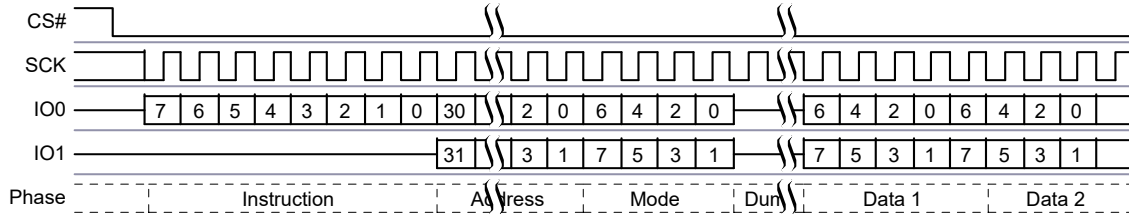
Figure 13. Dual I/O Command
