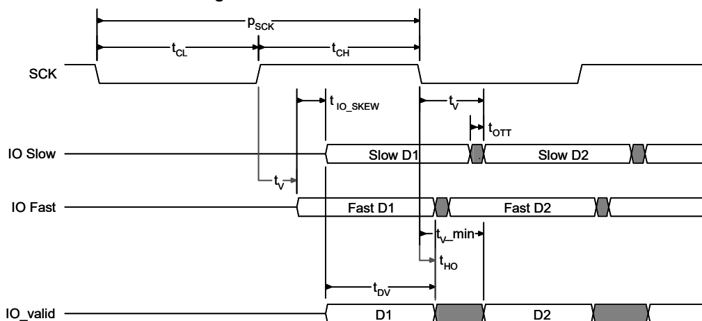
Figure 38. SPI DDR Data Valid Window
