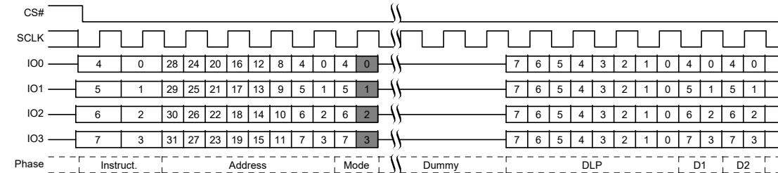
Figure 17. DDR Quad I/O Read Command QPI Mode
