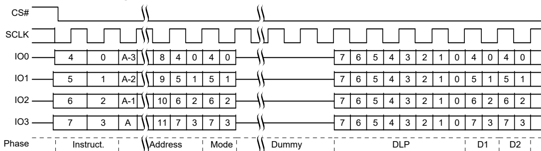
Figure 86. DDR Quad I/O Read Initial Access QPI Mode
