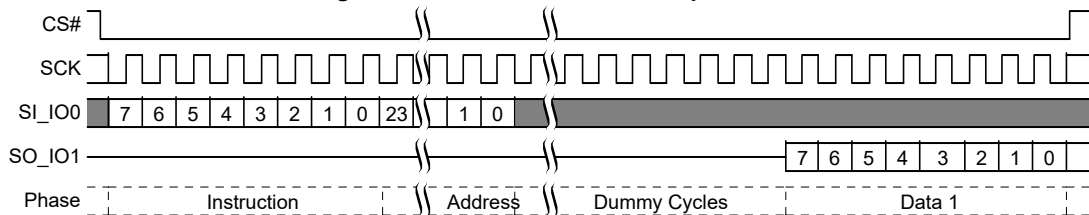
Figure 49. RSFDP Command Sequence
