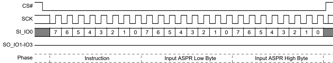
Figure 105. ASPP Command
