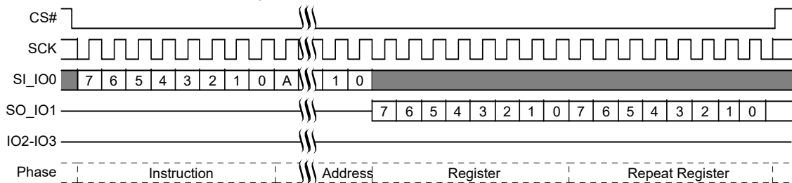
Figure 106. DYBRD Command Sequence
