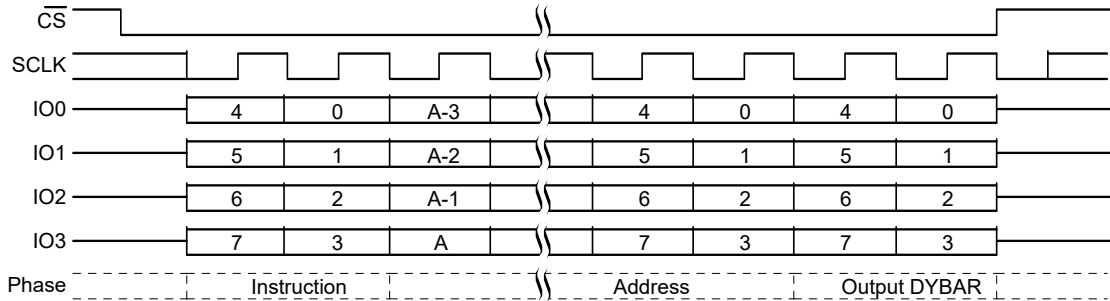
Figure 107. DYBRD QPI Mode Command Sequence
