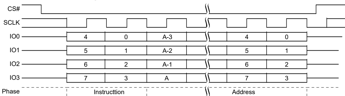
Figure 98. EES QPI Mode Command Sequence
