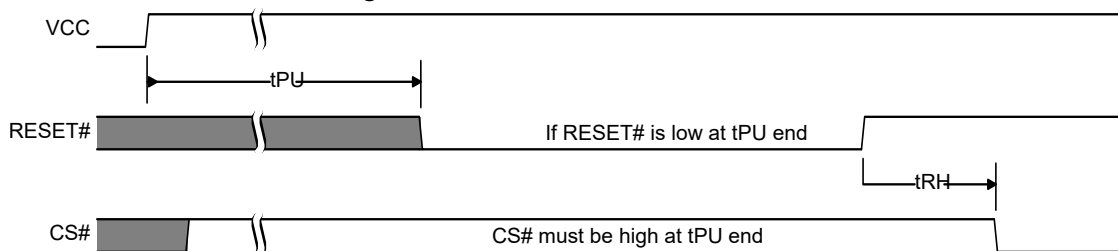
Figure 25. Reset low at the end of POR
