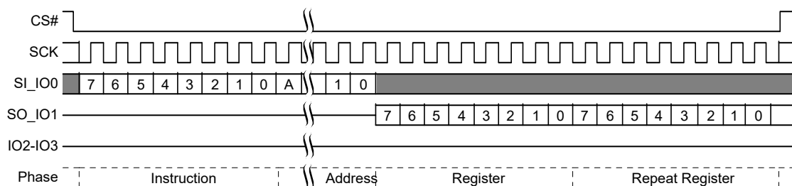
Figure 110. PPB Read Command Sequence
