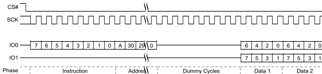
Figure 78. Dual Output Read Command Sequence
