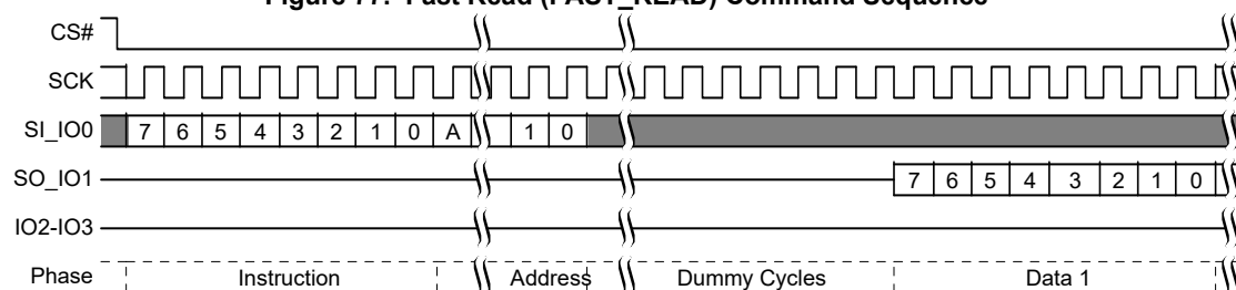
Figure 77. Fast Read (FAST_READ) Command Sequence
