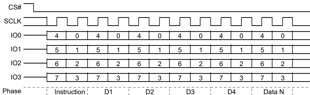
Figure 46. Read Identification (RDID) QPI Mode Command
