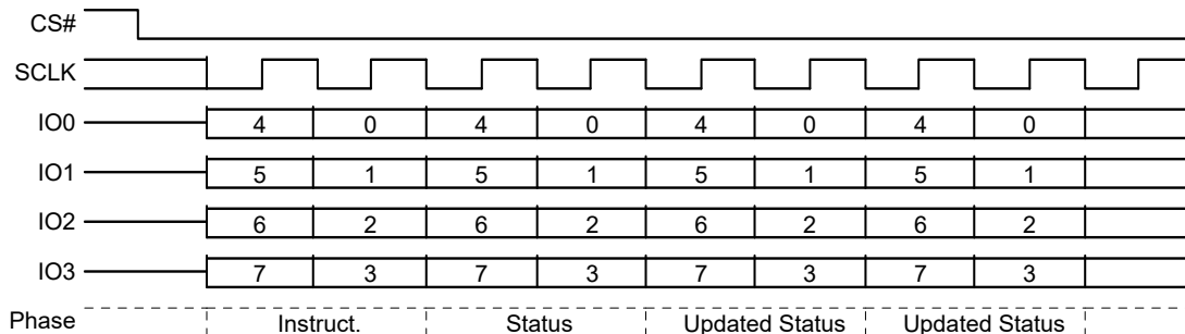
Figure 54. Read Status Register-1 (RDSR1) QPI Mode Command
