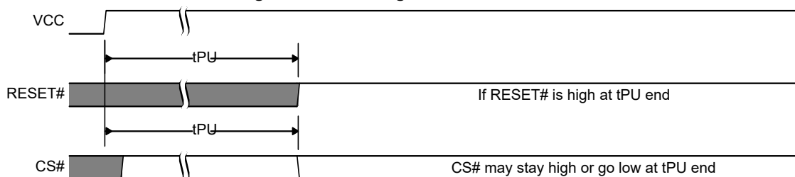
Figure 26. Reset high at the end of POR
