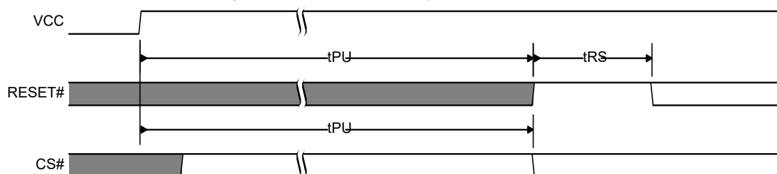
Figure 27. POR followed by Hardware Reset
