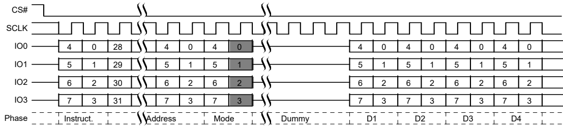
Figure 15. Quad I/O Read Command in QPI Mode
