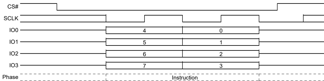
Figure 62. Write Disable (WRDI) Command Sequence QPI Mode
