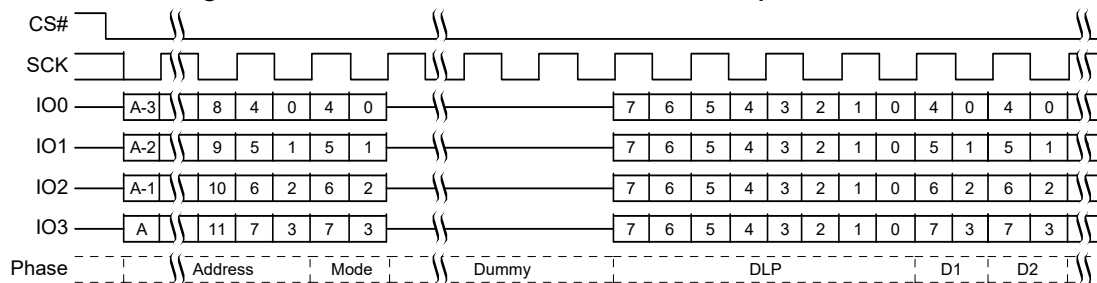
Figure 87. Continuous DDR Quad I/O Read Subsequent Access
