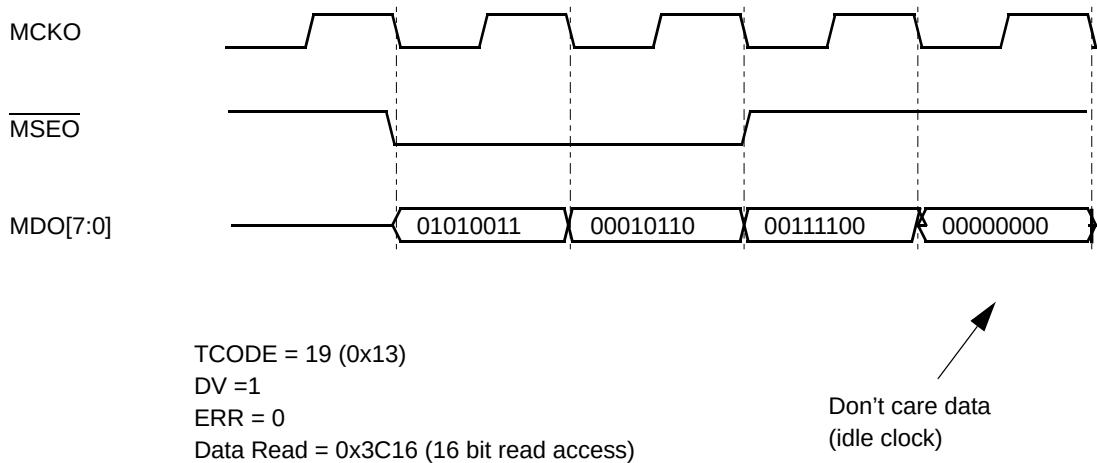
Figure 23-67. Upload/Download Information Message
