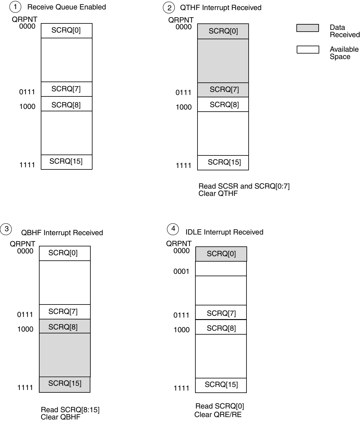
Figure 14-41. Queue Receive Example for 17 Data Bytes
