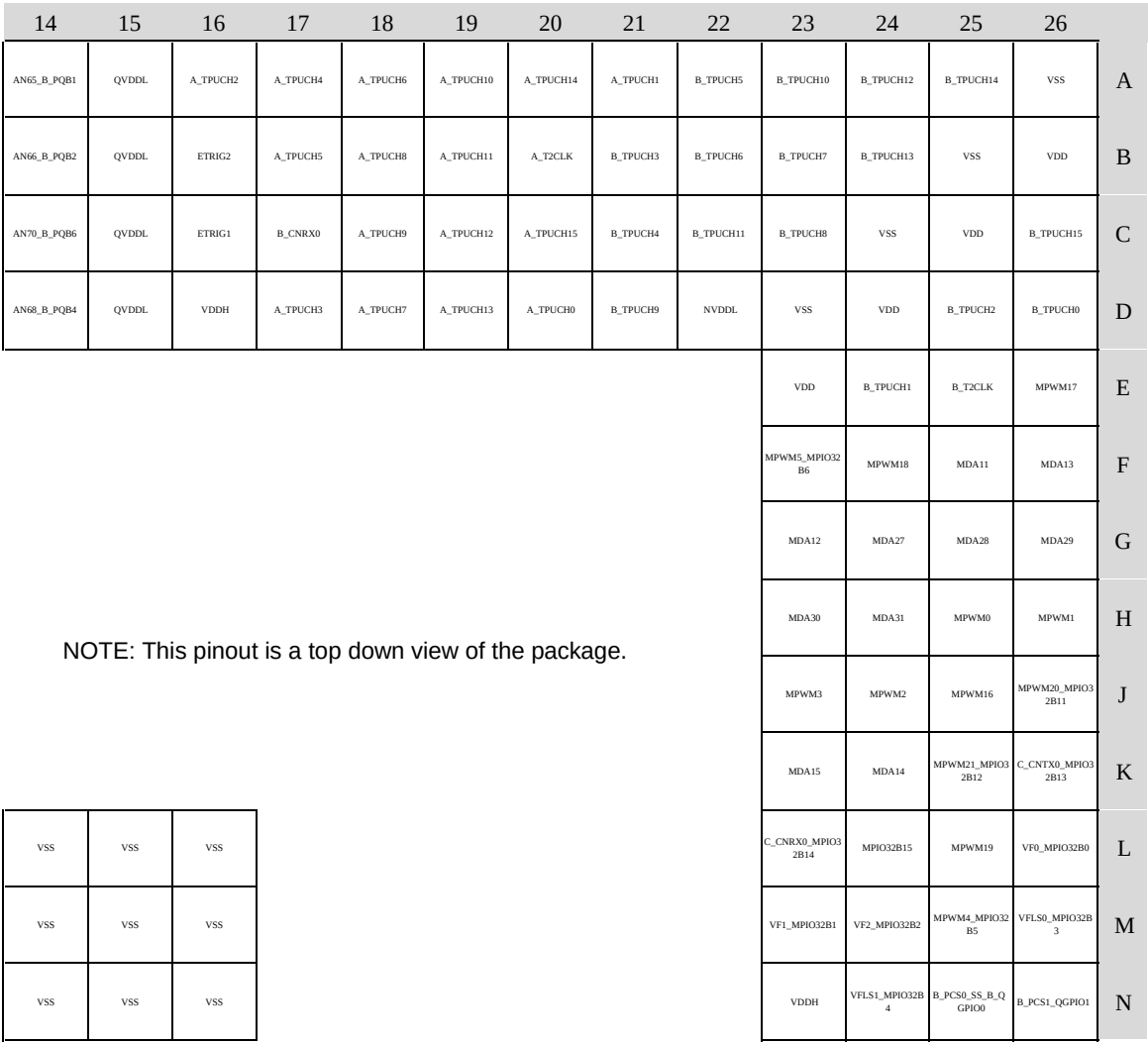
Figure F-67. MPC565 Ball Map (Black and White, page 3)
