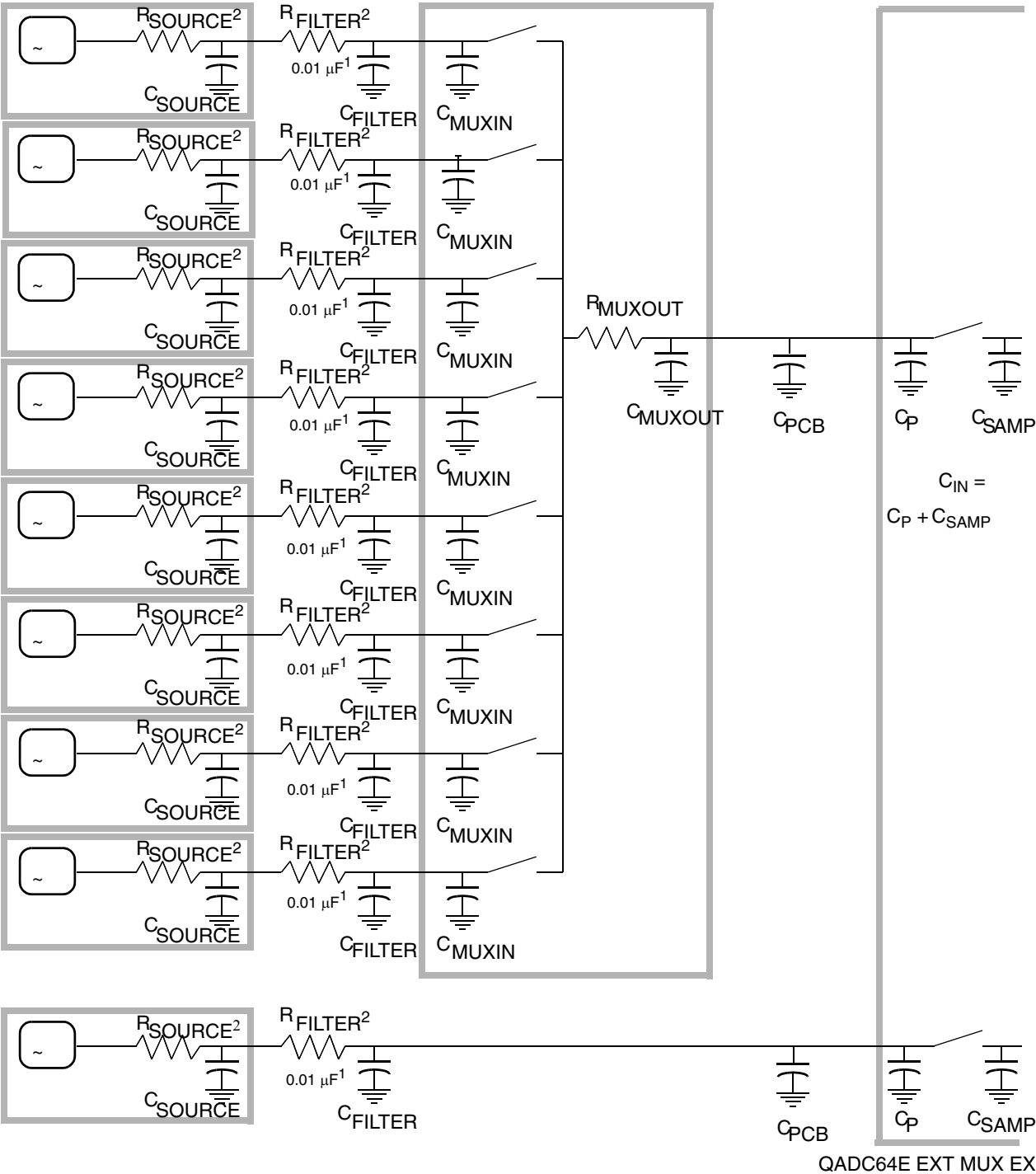
Figure 13-52. External Multiplexing of Analog Signal Sources
