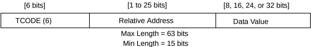
Figure 23-44. Data Read Message Format
