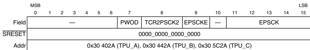
Figure 18-22. TPUMCR3 — TPU Module Configuration Register 3
