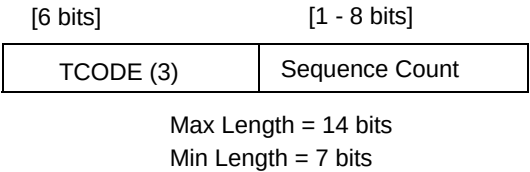
Figure 23-18. Direct Branch Message Format
