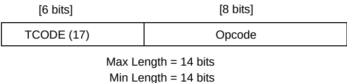
Figure 23-55. Read Register Message
