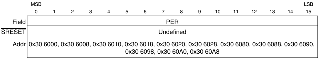
Figure 17-26. MPWMSM Period Register (MPWMPERR)
